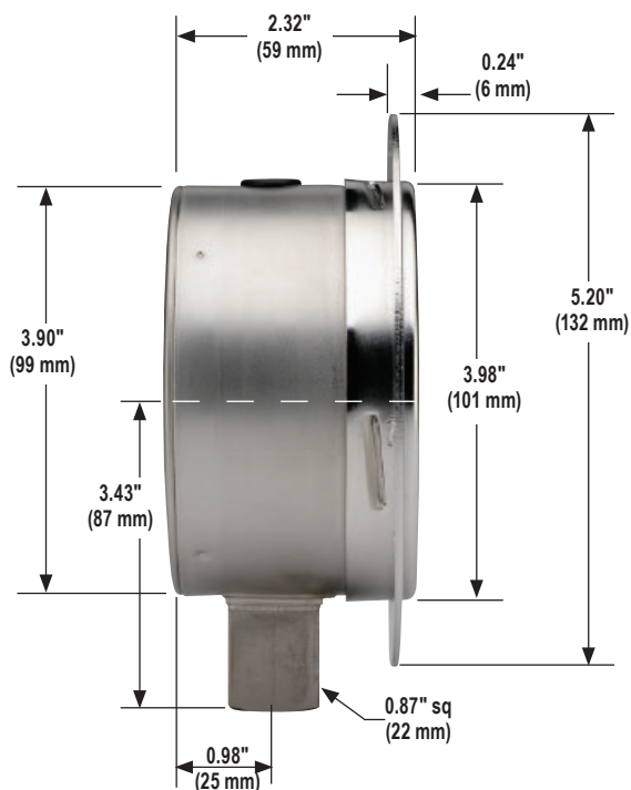
40-402/502 Front Flange
