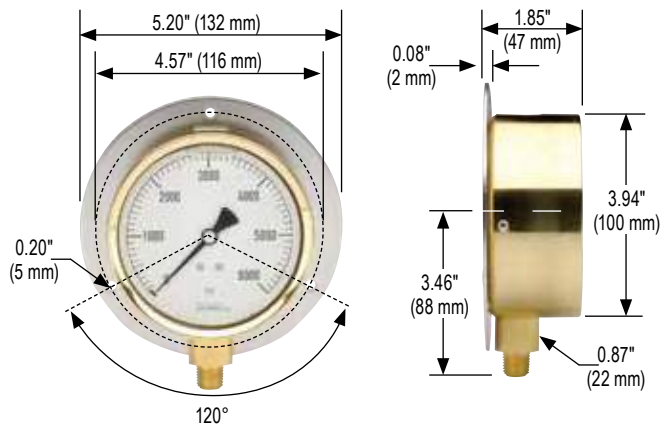
40-300 Rear Flange
