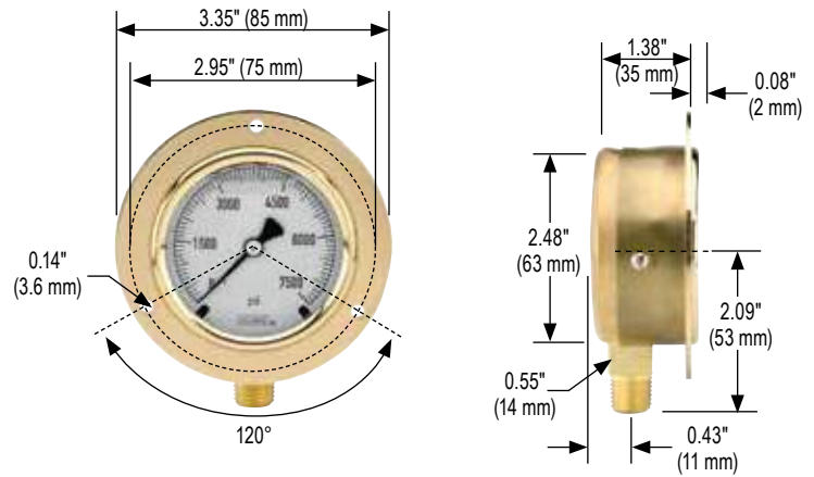
25-300 Front Flange
