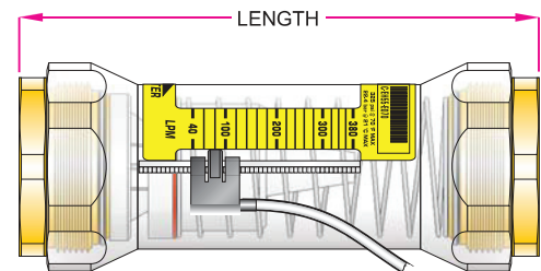
EZ-VIEW Flow Meter (with Flow-Apert Reed Switch)
