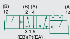
double solenoid pilot 2 position 4-way
