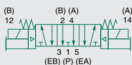
double solenoid pilot 3 position 4-way open center
