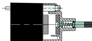
Extended Knurled Rod Non-Locking Override with light
