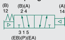
PA double air pilot 2 position 4-way with spring offset
