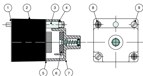
Flush Non-Locking Override with light (standard)
