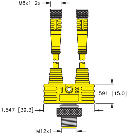
VB2-FSM 4.4/2RK 4T-*/*
