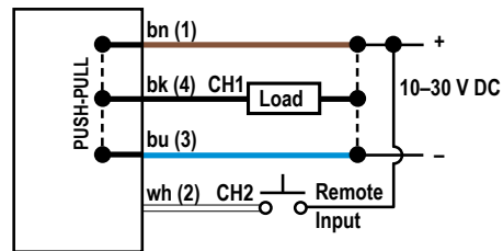
Figure 12. Channel 2 as remote input
