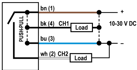
Figure 11. Channel 2 as PNP discrete or PFM output
